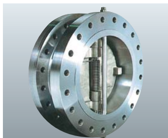
DCF Dual plate check valve(FLANGE Type)
