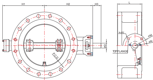
FLANGE TYPE
