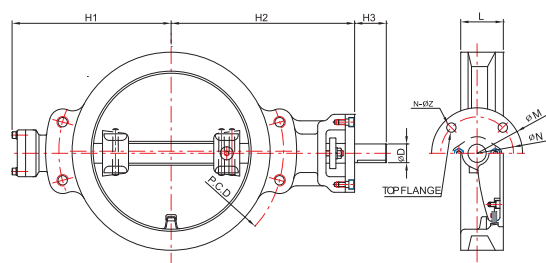
WAFER TYPE
